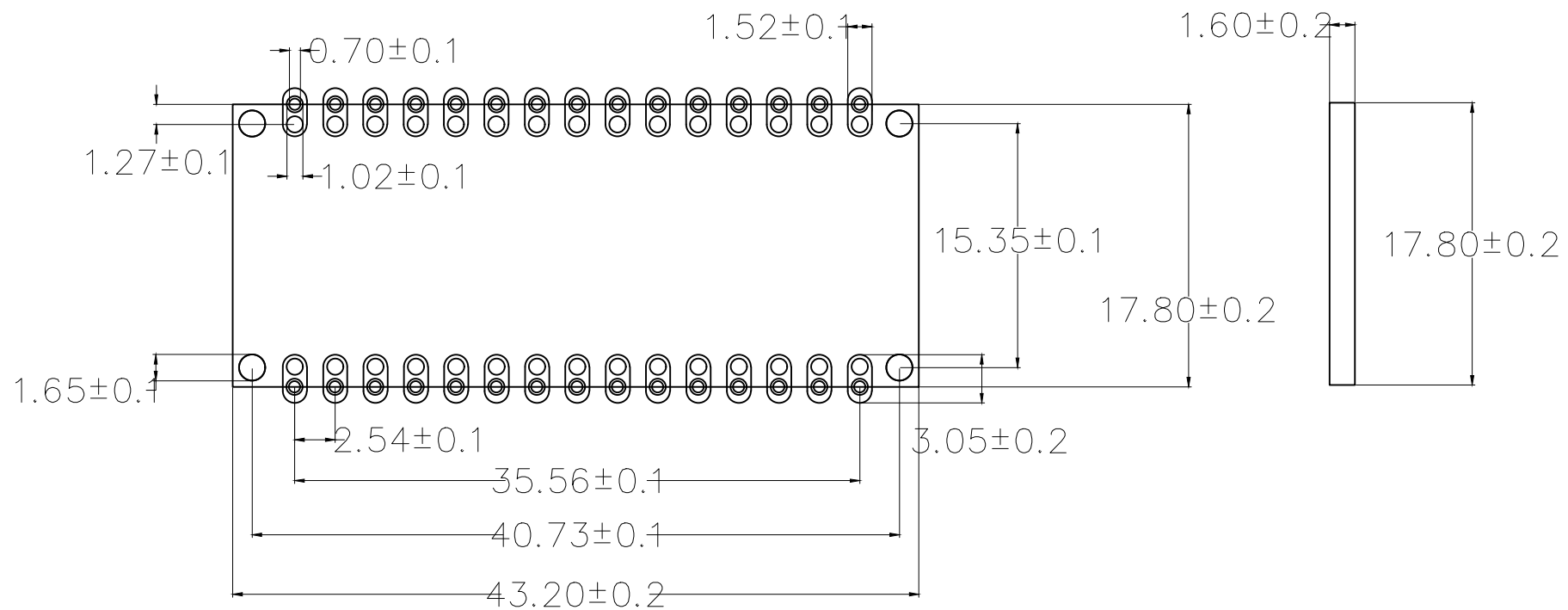
Side View
